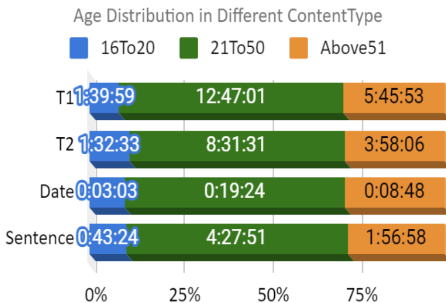
Figure 5: Age Distribution in different Content Types of Maithili Corpus
